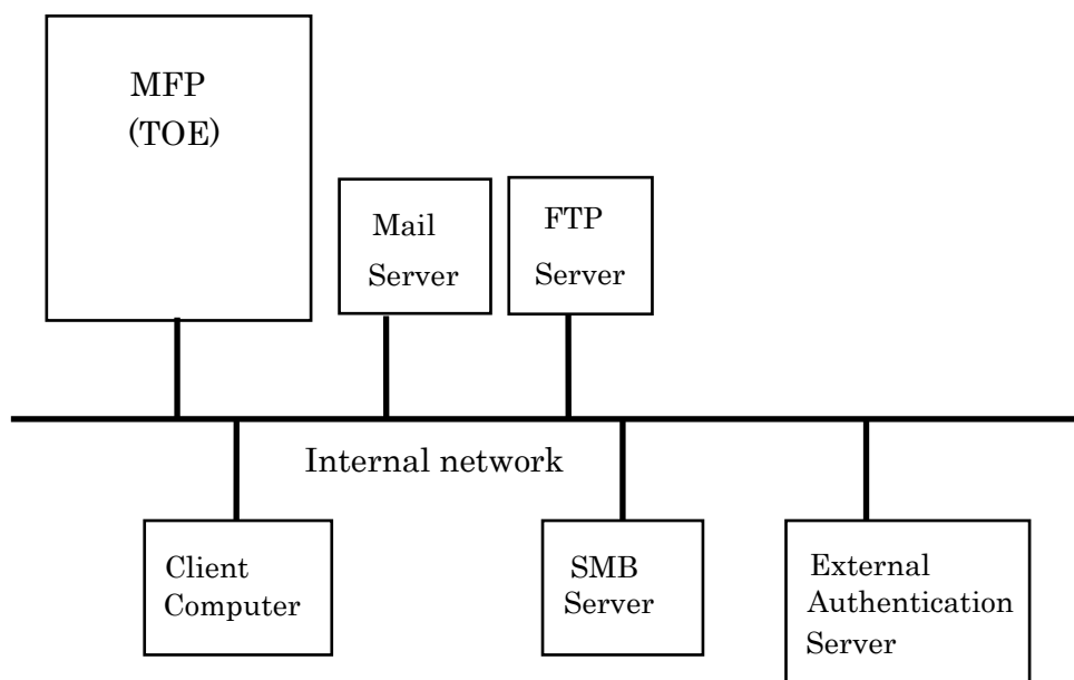
Figure 7-1 Configuration of the Developer Testing
