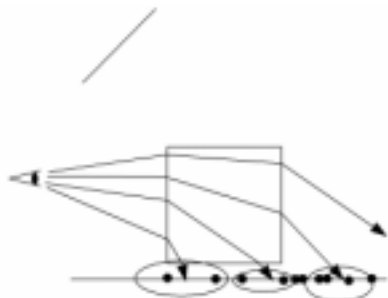
Fig.5 Caustics Rays
