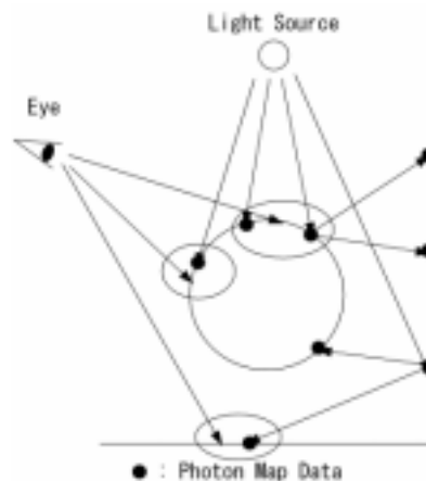
Fig.2 Photon Mapping
