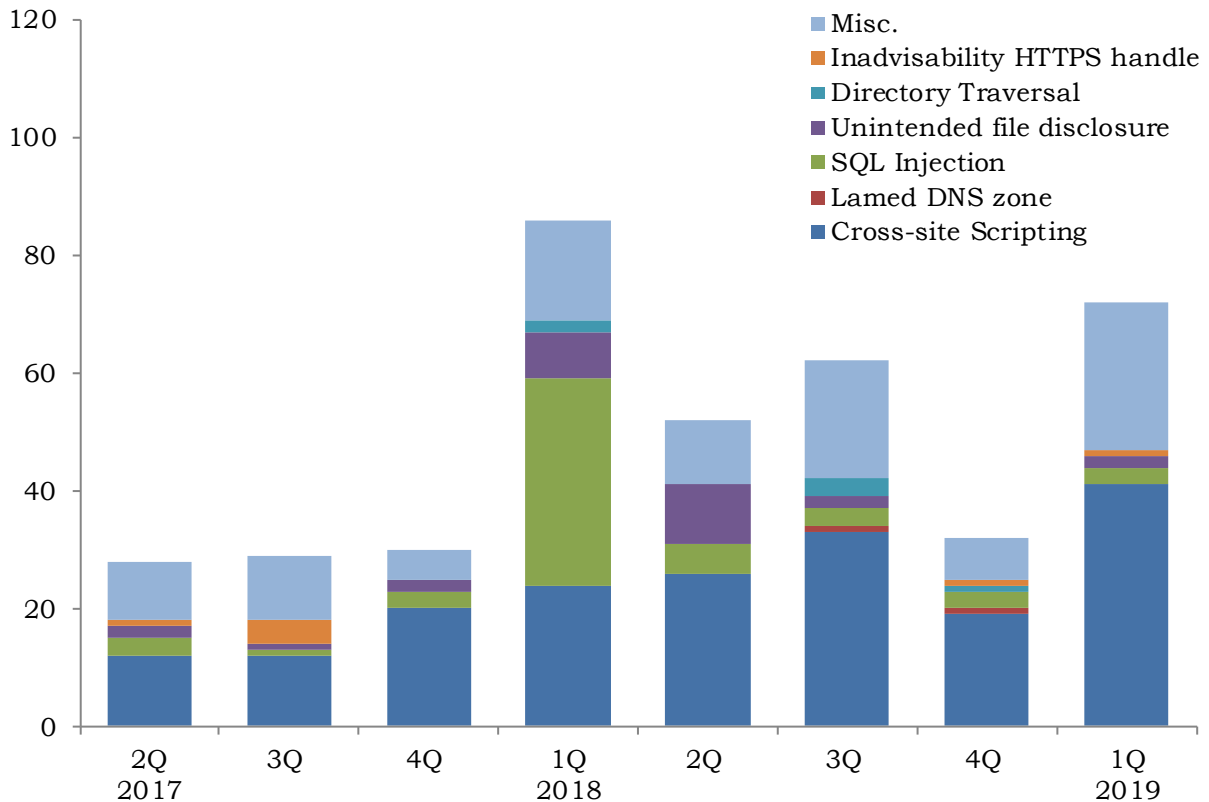
Chart 3-2: Shift in Number of Vulnerabilities in Websites by Type (from April 1 2017, to the End of March, 2019)
