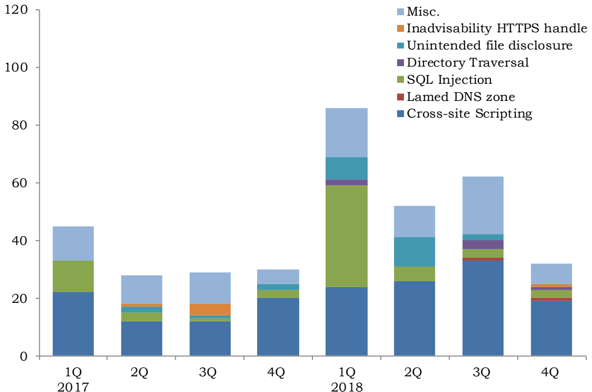
Chart 3-2: Shift in Number of Vulnerabilities in Websites by Type (from January 1 2017, to the End of December, 2018)
