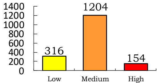
Chart 2-1 : Severity of Vulnerabilities in Software Products on JVN Several reports may be summarized in one on JVN. (from Initial Acceptance to the end of December, 2018)
