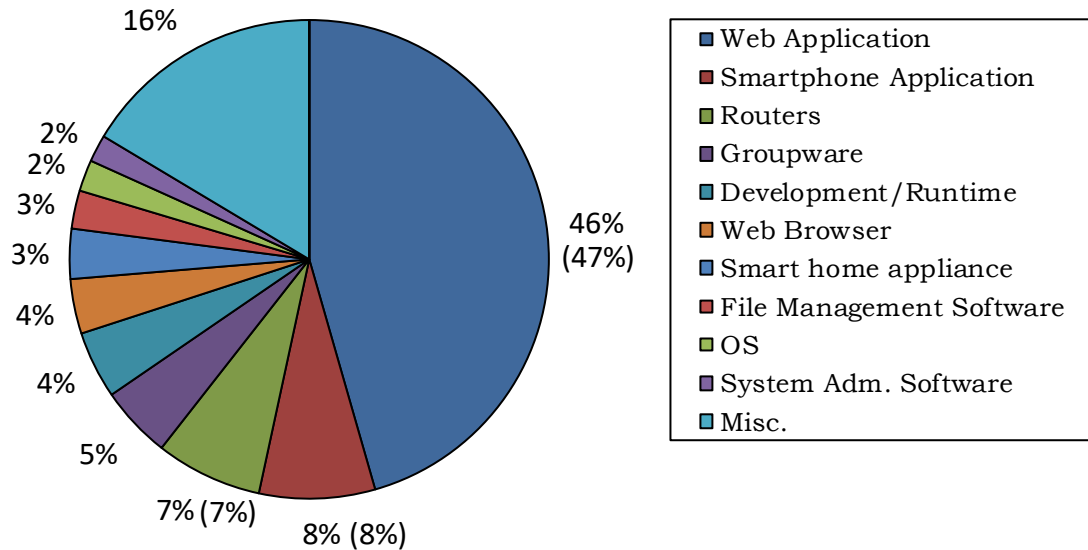
Chart 2-2: Breakdown of the Vulnerabilities in Software Products (from July 8, 2004 to the end of March, 2018)
