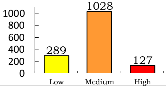
Chart 2-1 : Severity of Vulnerabilities in Software Products on JVN Several reports may be summarized in one on JVN. (from Initial Acceptance to the end of June, 2017)
