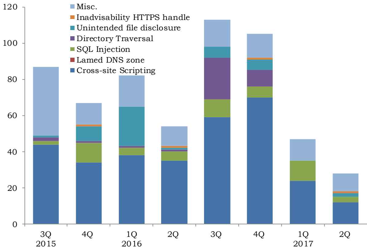
Chart 3-2: Shift in Number of Vulnerabilities in Websites by Type (from July 1 2015, to the End of June, 2017)
