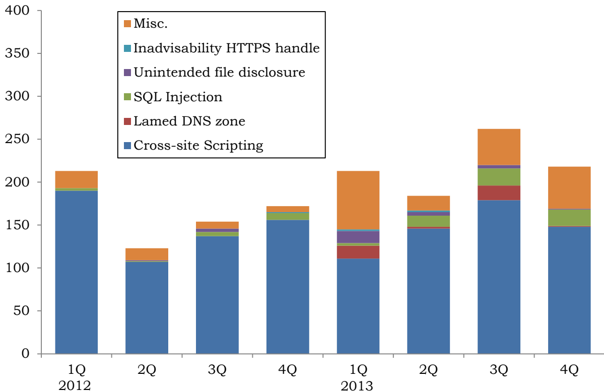
Chart 3-2: Shift in Number of Vulnerabilities in Websites by Type (from January 1 2011, to the End of December, 2013)
