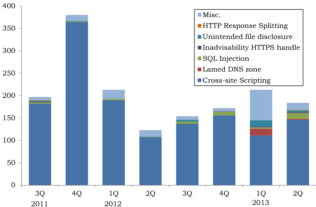
Chart 3-2: Shift in Number of Vulnerabilities in Websites by Type (from July 1 2011, to the End of June, 2013)
