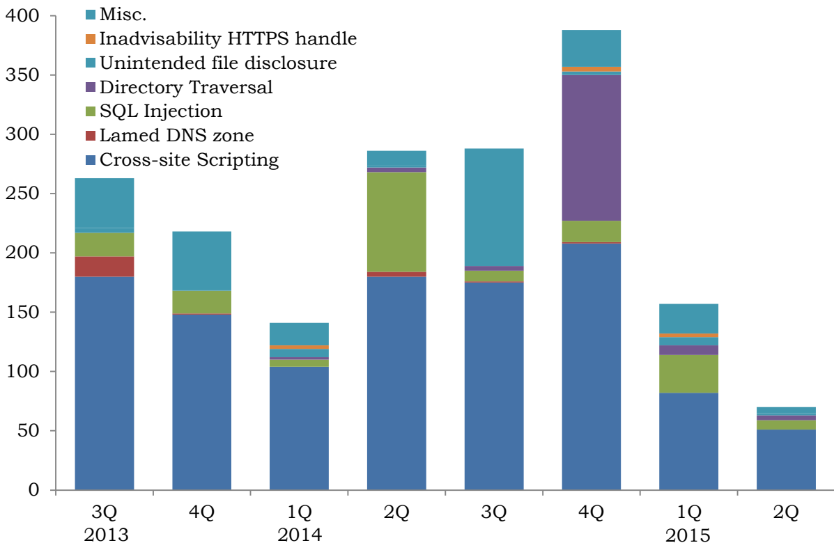
Chart 3-2: Shift in Number of Vulnerabilities in Websites by Type (from July 1 2013, to the End of June, 2015)
