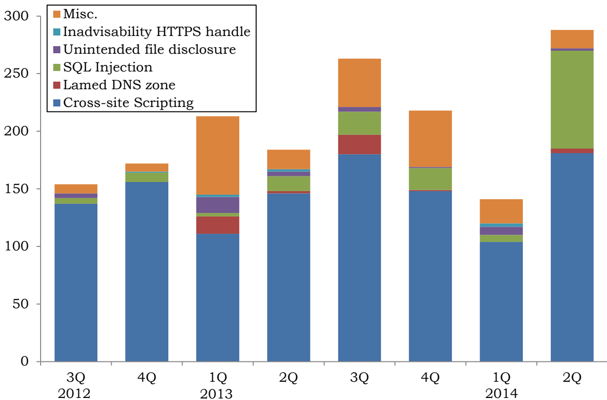
Chart 3-2: Shift in Number of Vulnerabilities in Websites by Type (from July 1 2012, to the End of June, 2014)
