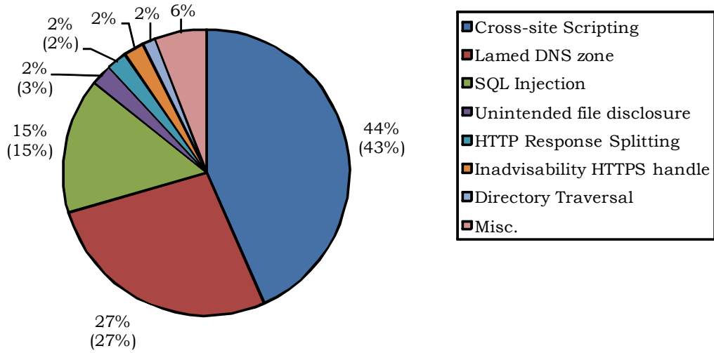
Chart 3-1: Breakdown of Vulnerabilities in Websites by Type (from July 8 2004, to the end of June, 2009)
