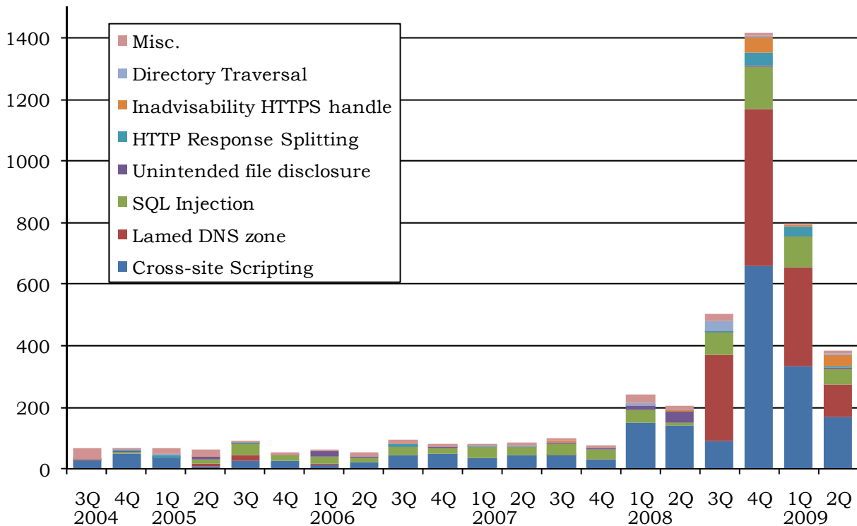
Chart 3-2: Shift in Number of Vulnerabilities in Websites by Type (from July 8 2004, to the End of June, 2009)
