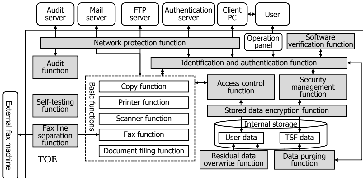
Figure 5-1 TOE boundary
