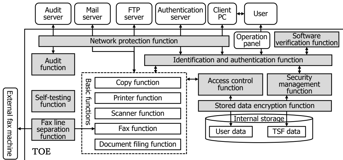
Figure 5-1 TOE boundary
