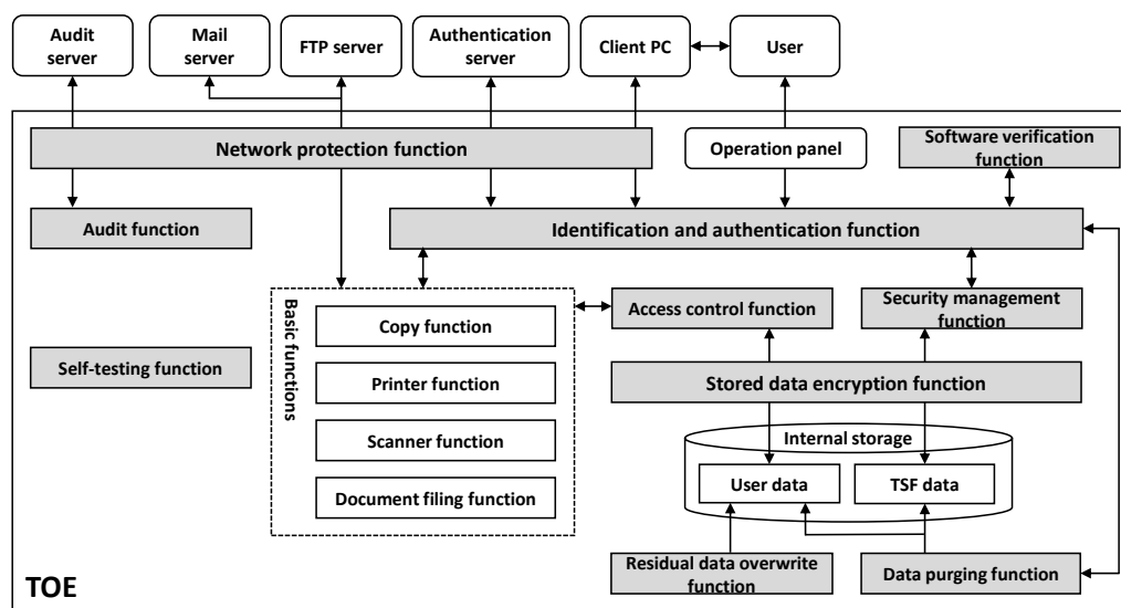
Figure 5-1 TOE boundary
