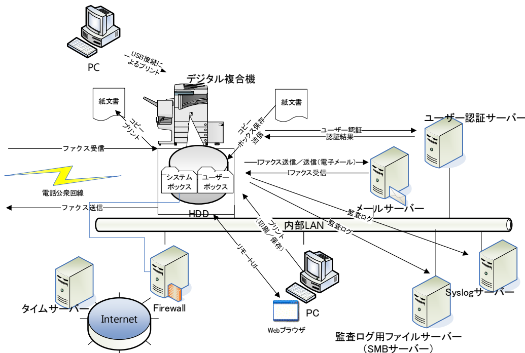
Figure 1 デジタル複合機< Canon imageRUNNER ADVANCE DX 717/617/527 Series with Fax > の運用環境
