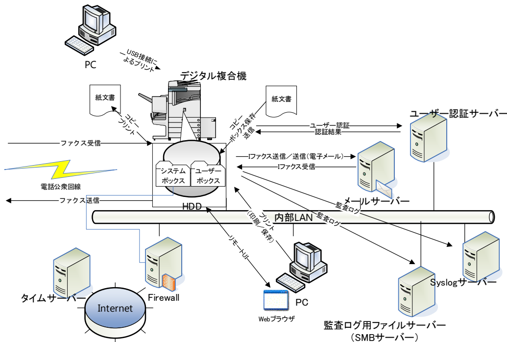
Figure 1 デジタル複合機< Canon imageRUNNER ADVANCE DX C477 Series with Fax>の運用環境
