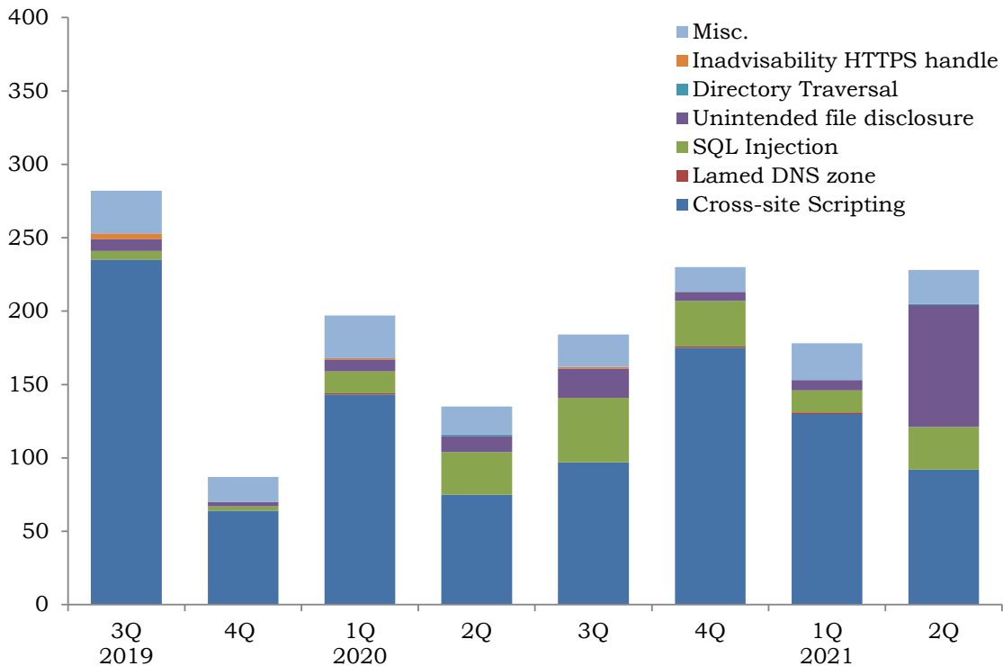
Chart 3-2: Shift in Number of Vulnerabilities in Websites by Type (from July 1 2019, to the End of June, 2021)
