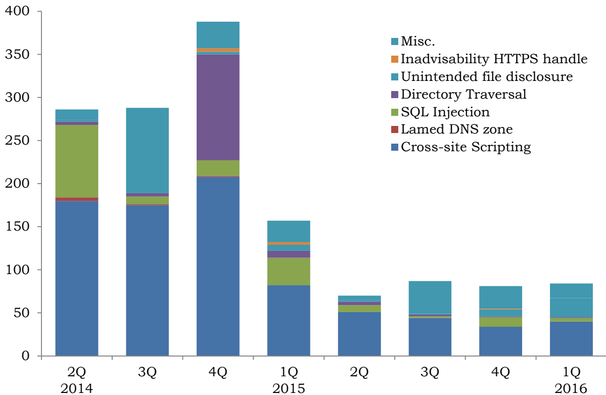
Chart 3-2: Shift in Number of Vulnerabilities in Websites by Type (from April 1 2014, to the End of March, 2016)
