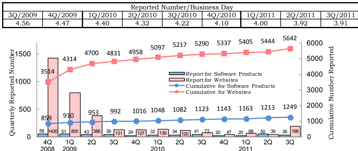
Chart 1-1: Quarterly Number of Vulnerability-related Information
