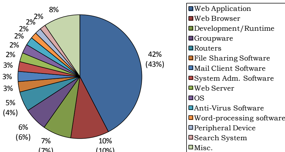
Chart 2-2: Breakdown for the Vulnerabilities in Software Products (from July 8, 2004 to the end of September, 2011)
