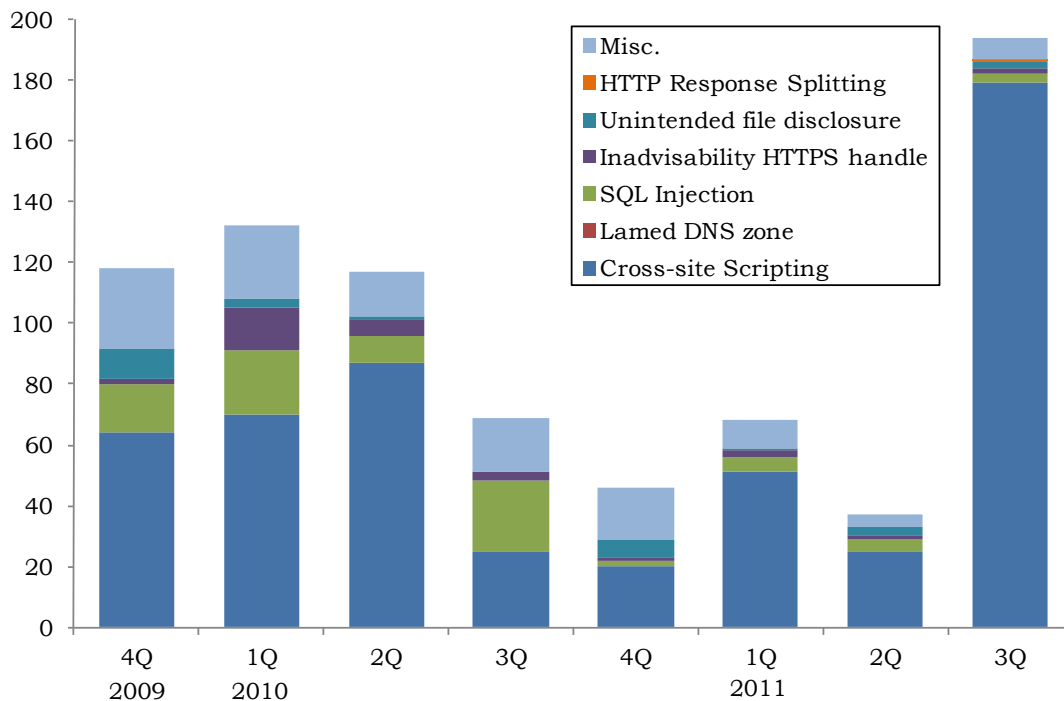
Chart 3-2: Shift in Number of Vulnerabilities in Websites by Type (from October 1 2009, to the End of September, 2011)
