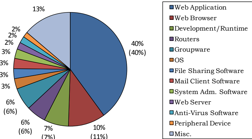
Chart 2-2: Breakdown of the Vulnerabilities in Software Products (from July 8, 2004 to the end of December, 2012)
