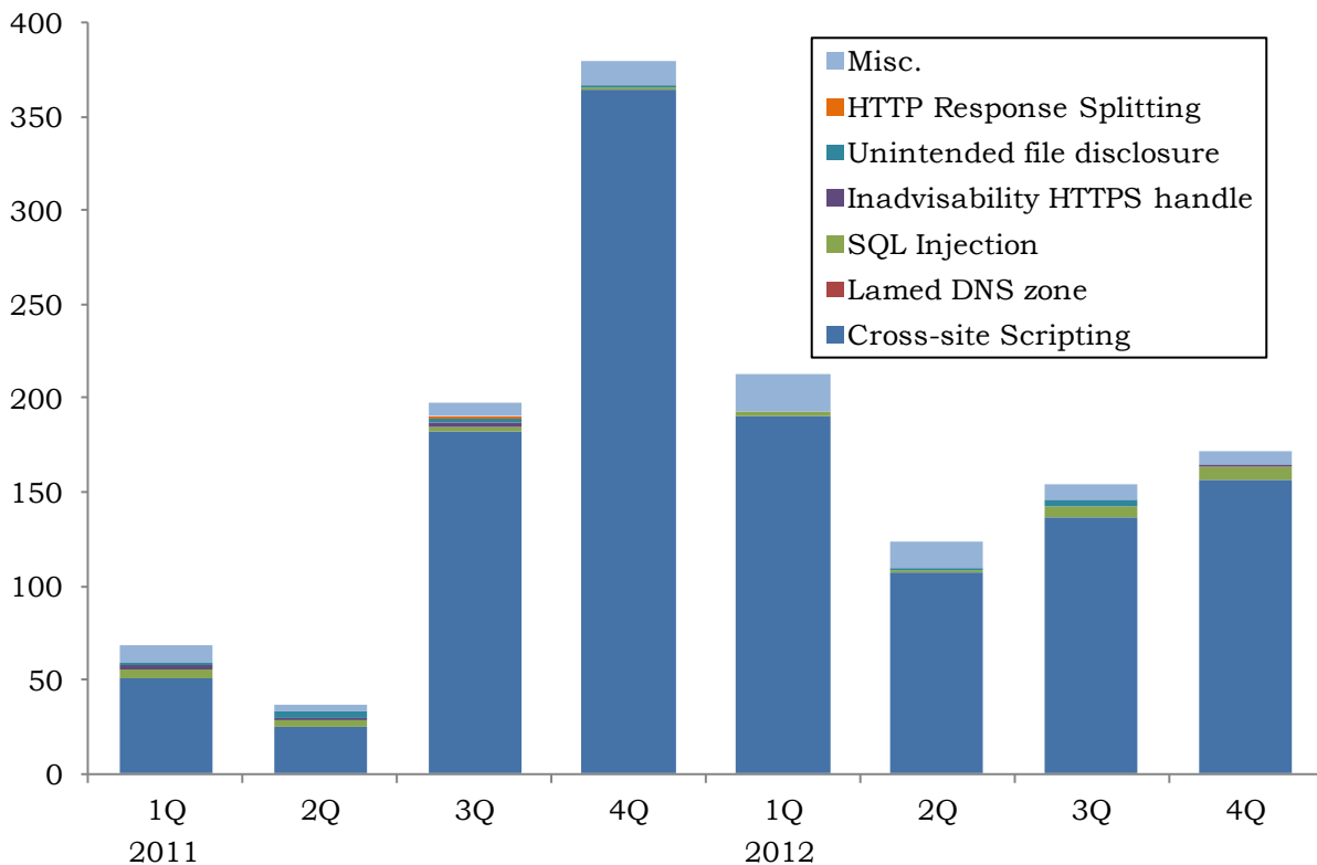
Chart 3-2: Shift in Number of Vulnerabilities in Websites by Type (from January 1 2011, to the End of December, 2012)
