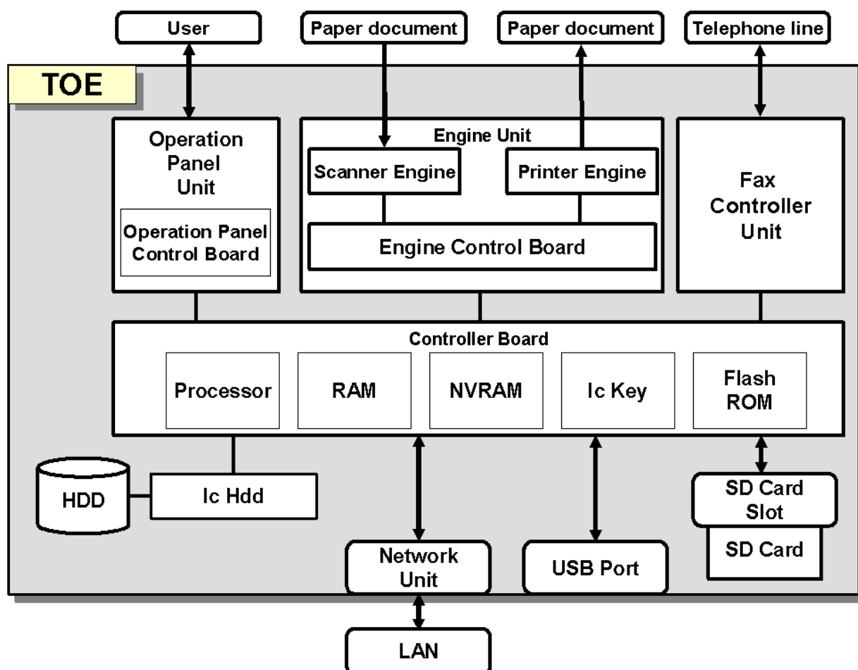
Figure 5-1 TOE boundary
