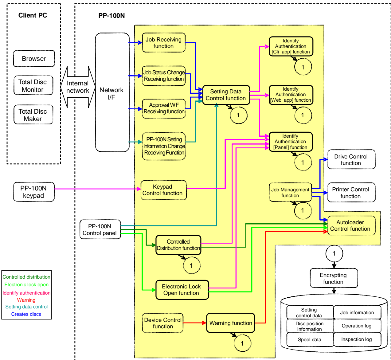
Figure 4: Logical Configuration
