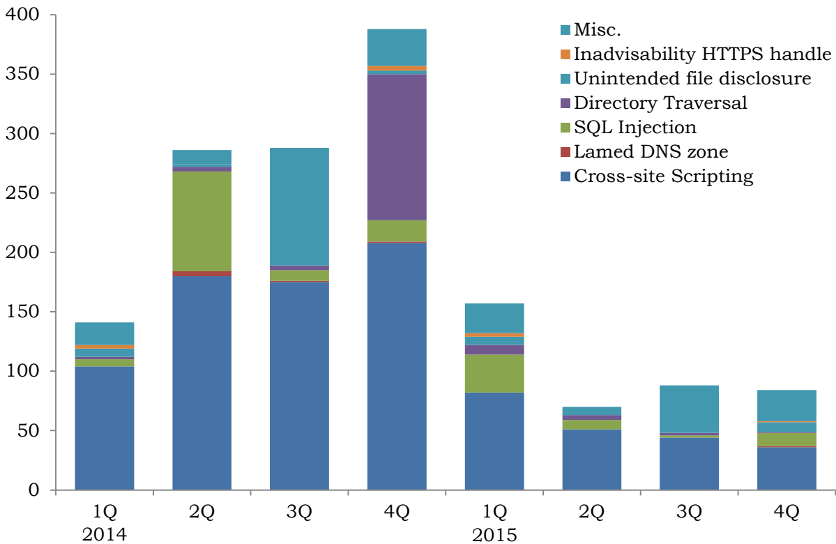
Chart 3-2: Shift in Number of Vulnerabilities in Websites by Type (from January 1 2014, to the End of December, 2015)
