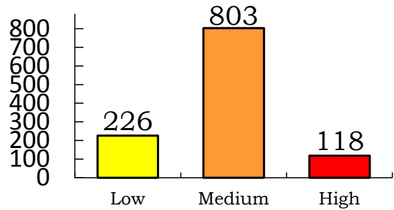
Chart 2-1 : Severity of Vulnerabilities in Software Products (from Initial Acceptance to the end of December, 2015)
