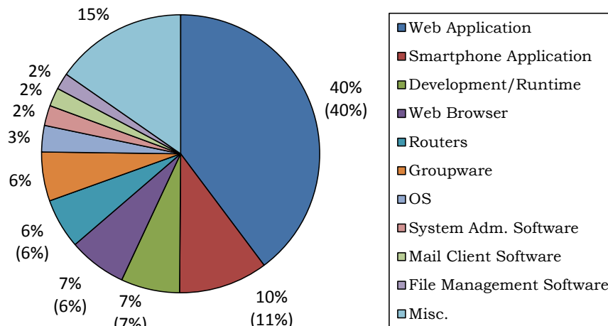
Chart 2-2: Breakdown of the Vulnerabilities in Software Products (from July 8, 2004 to the end of December, 2015)
