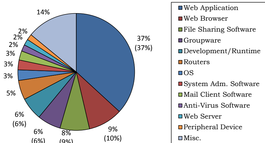
Misc. in this graph includes Software for Database, etc. (Breakdown of 1543: Numbers in parenthesis are for the previous quarter)
