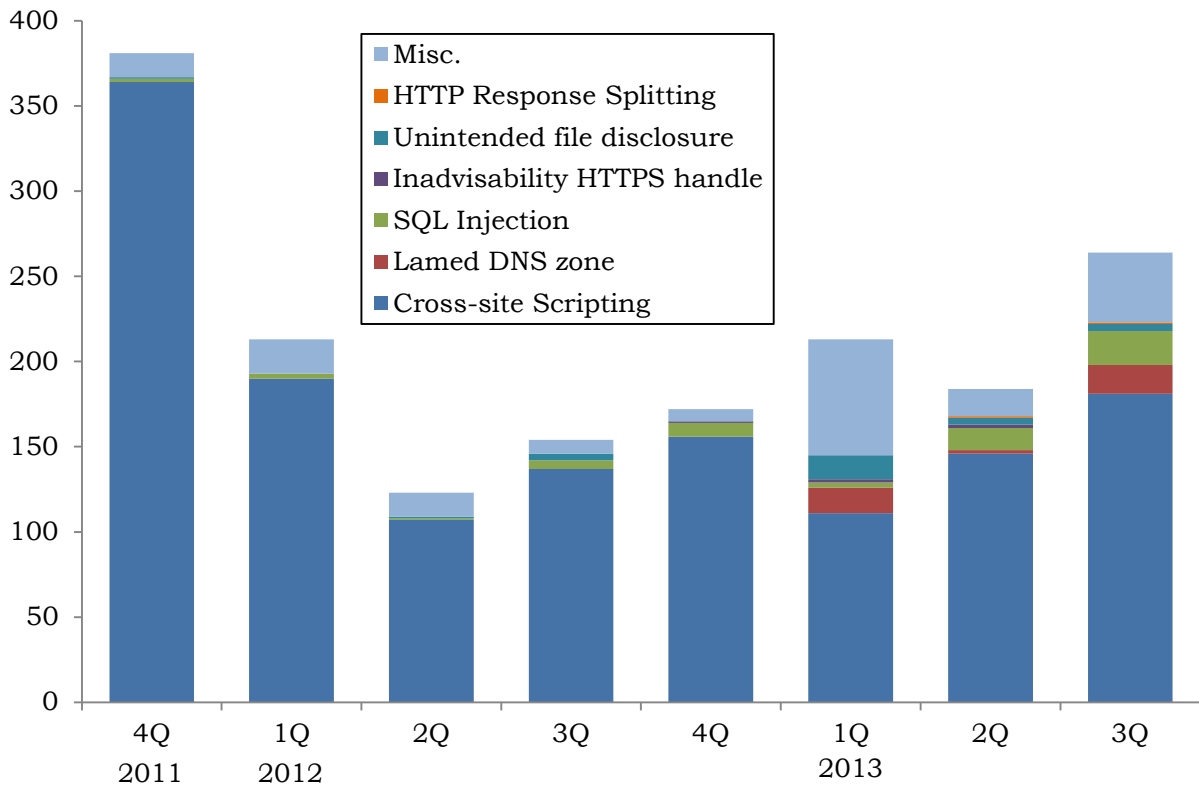
Chart 3-2: Shift in Number of Vulnerabilities in Websites by Type (from October 1 2011, to the End of September, 2013)
