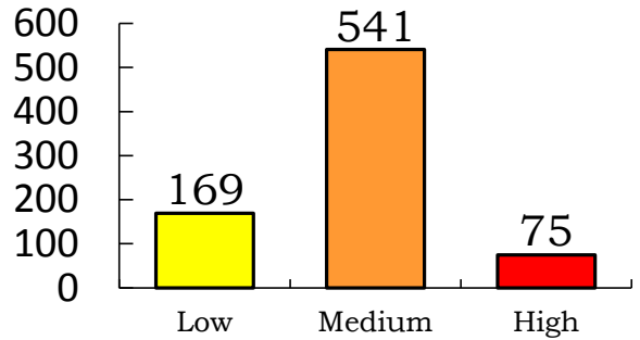
Chart 2-1 : Severity of Vulnerabilities in Software Products (from Initial Acceptance to the end of September, 2013)
