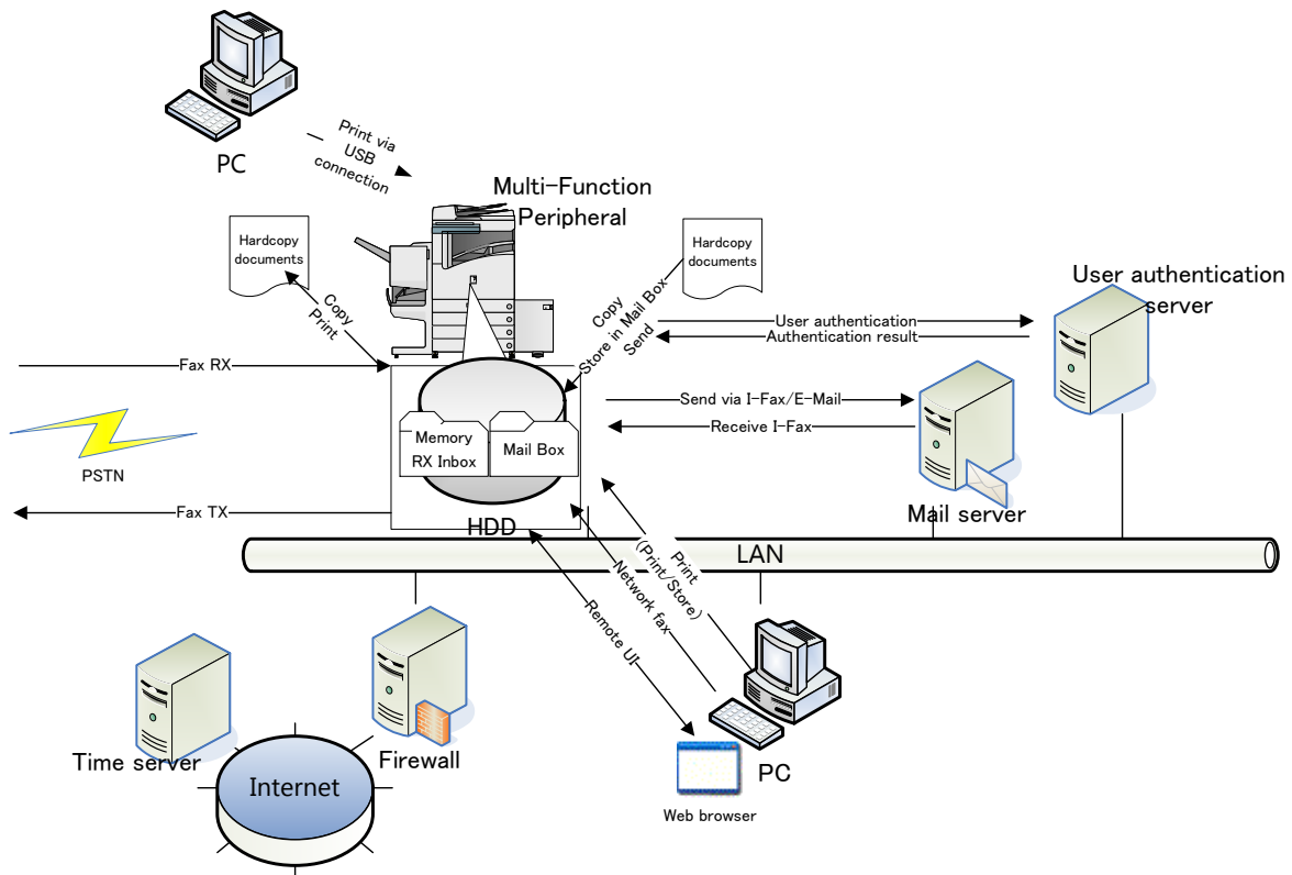
Figure 1 The assumed operational environment of the MFP < Canon imageRUNNER ADVANCE C355/C255 Series >
