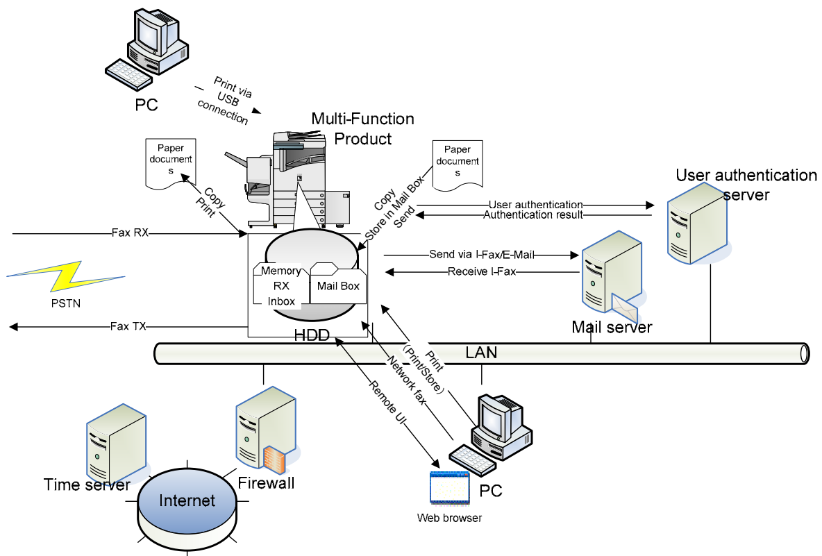
Figure 1 The assumed operational environment of the MFP < Canon imageRUNNER ADVANCE 4200 Series >
