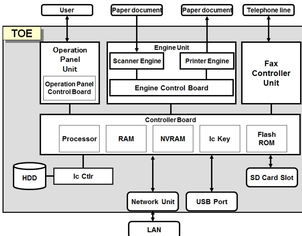
Figure 5-1 TOE Boundary
