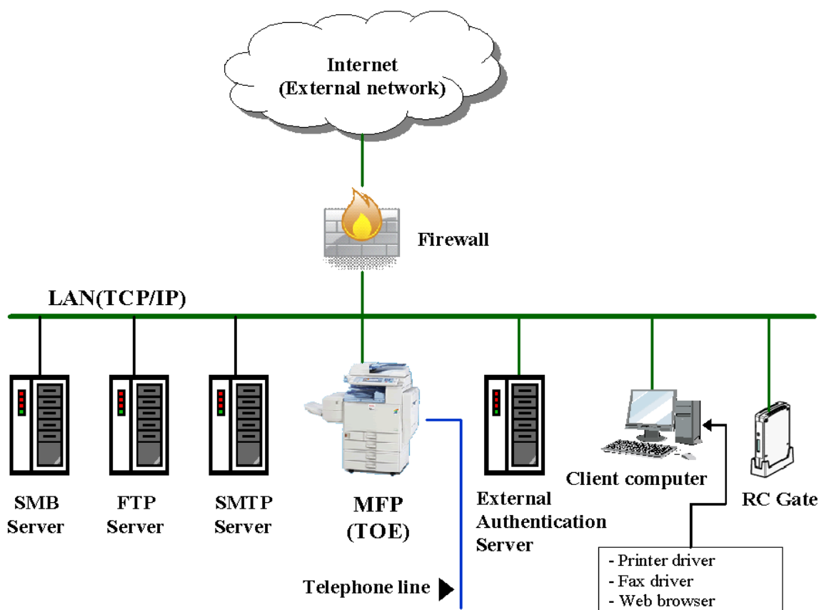
Figure 4-1 Operational Environment and Configuration
