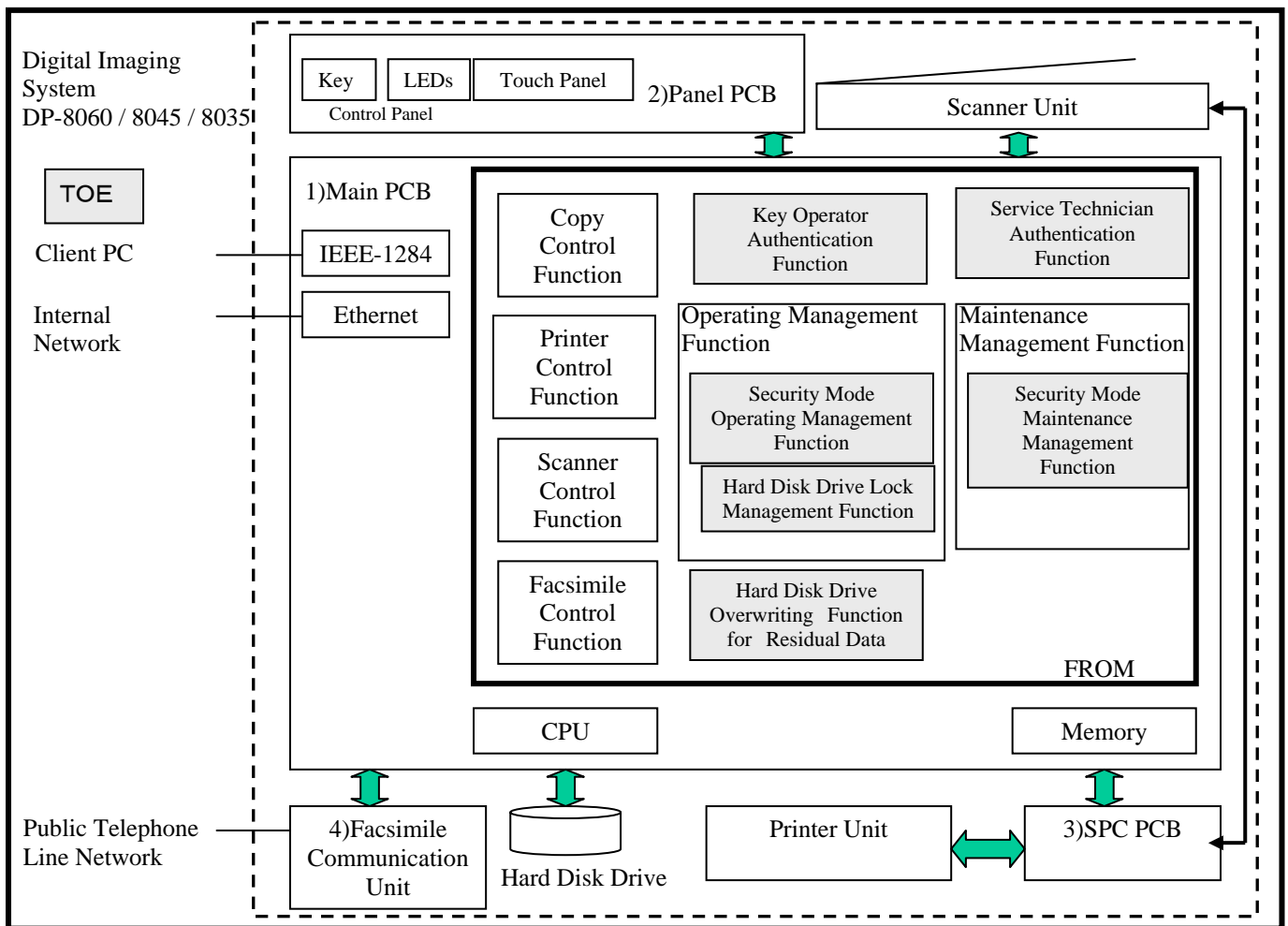
Fig. 2 Physical Configuration of Digital Imaging System DP-8060 / 8045 / 8035 and TOE
