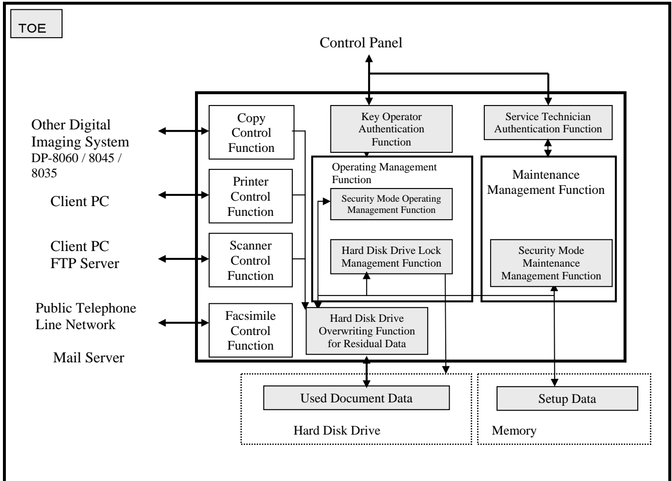
Fig. 3 Logical Configuration of Digital Imaging System DP-8060 / 8045 / 8035 and TOE
