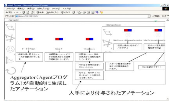
RSS Reader
